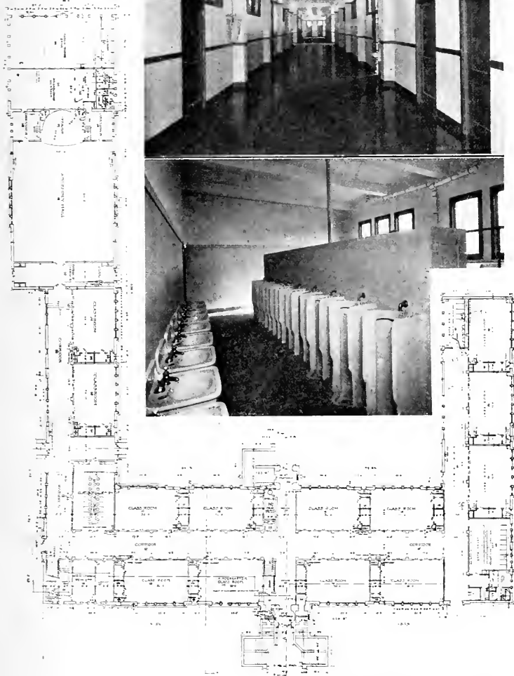
FIRST FLOOR PLAN, MAIN CORRIDOR AND BOYS' LAVATORY, DURANT SCHOOL, OAKLAND
